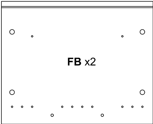
484x390x15mm
